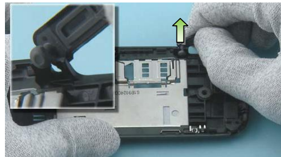
18) Remove EF II COVER by pulling it out gently in the direction shown.
