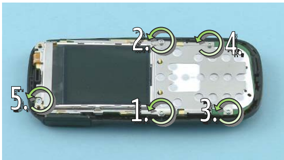
5) After placing the ENGINE MODULE, tighten the five Torx+ 4 screws to the torque of 18 Ncm in the order shown.
