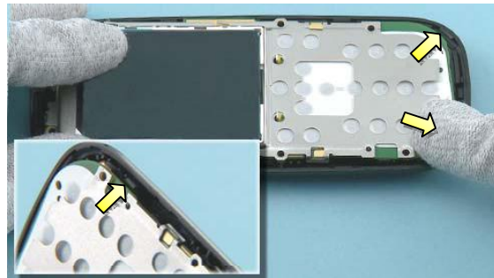
4) Then press gently on the lower ends of the ENGINE MODULE to lock with the two snaps on the D-COVER.
