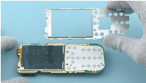
21) Remove the UI SHIELDING.
